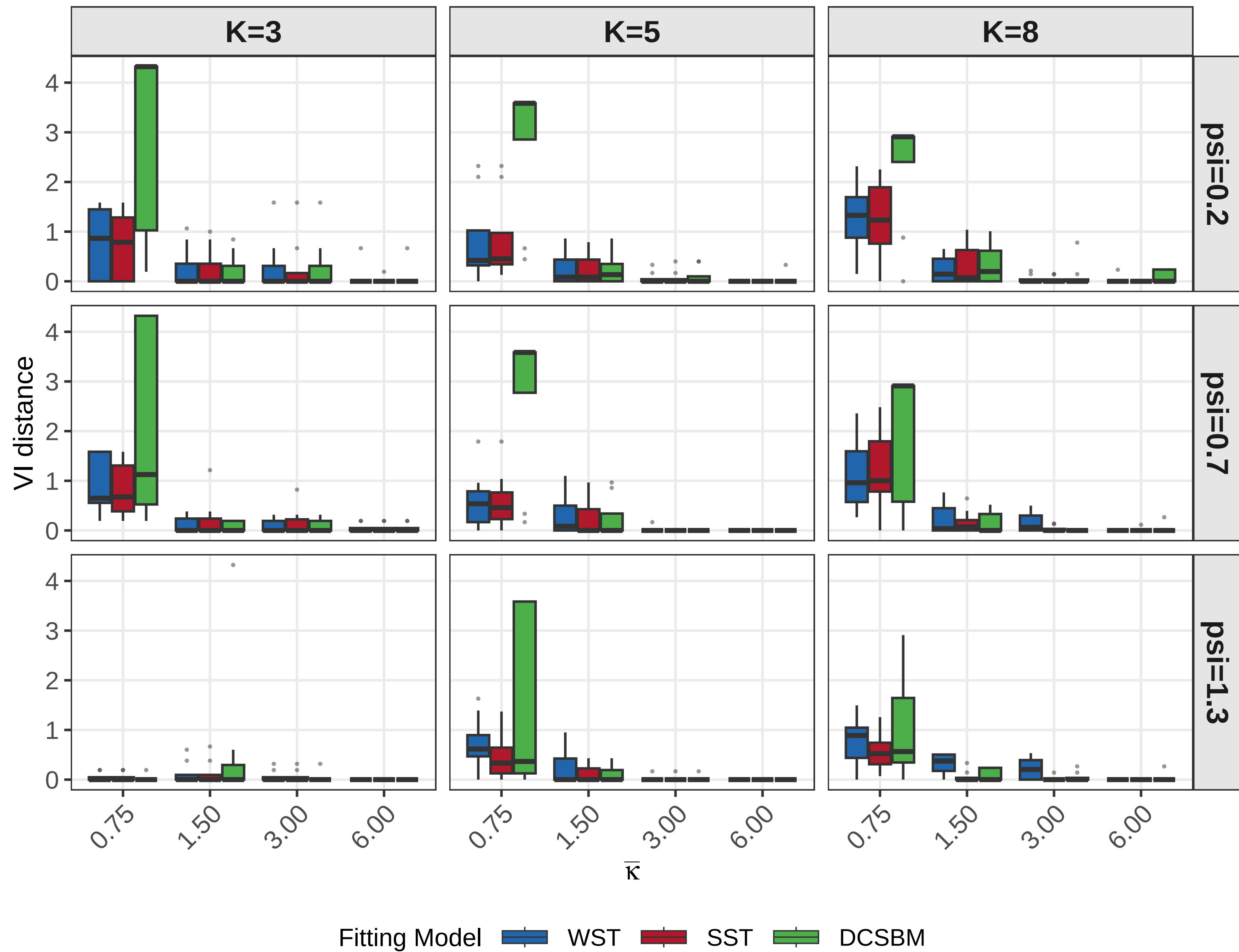
Variation of Information: All Generating Models
